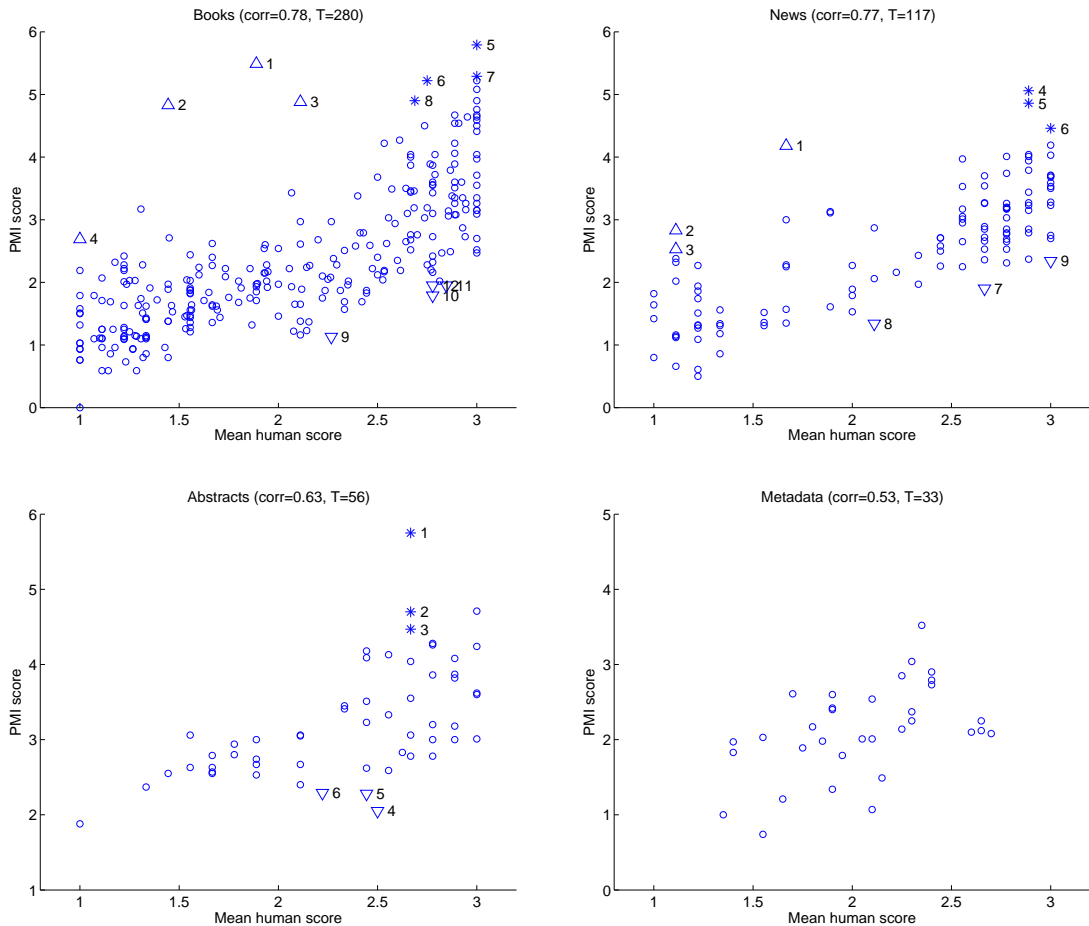
Figure 3: Scatter plots showing PMI score vs. mean human score for topics in the four collections. Annotated topics show outliers that either overpredict PMI at low scores ( \Delta ), overpredict PMI at high scores (*), or underpredict PMI at high scores ( \nabla ). We see relatively good agreement between the PMI score and the human score (as indicated by the correlation values) across a wide variety of text collections.
