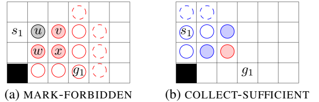
Figure 4: Explaining c_i \geq 6 . Filled nodes are obstacles, red nodes are explored by \text{MARK-FORBIDDEN} , blue nodes explored by \text{COLLECT-SUFFICIENT} . Dashed nodes were pruned due to H .
