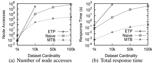
Fig. 29 Maintenance cost with the effect of dataset sizes
