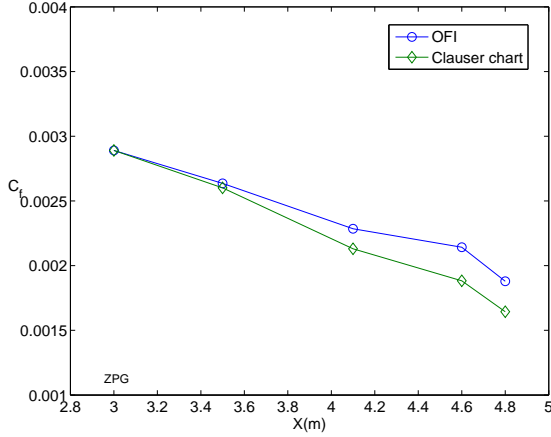
Figure 4: Friction coefficient at a matched Re_\tau \simeq 1850 .
