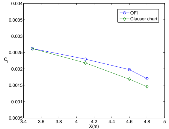
Figure 3: Friction coefficient for matched K \simeq 15.2 with increasing Re_\tau .
