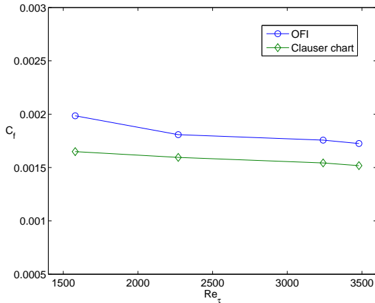
Figure 5: Friction coefficient for matched \beta \simeq 4.4 with an increasing Re_\tau .
