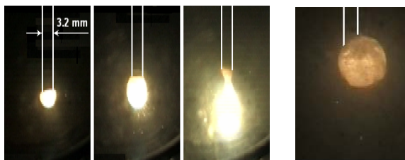
(a) t = -0.92 \text{ s} t = -0.64 \text{ s} t = -0.36 \text{ s} (b) t = 1.50 \text{ s} Figure 4. A metallic rod sample burning in (a) normal gravity and (b) in reduced gravity.
