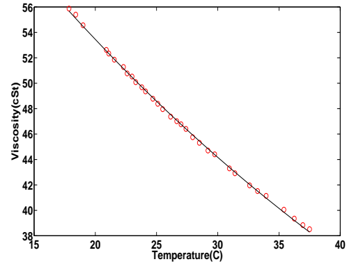
Figure 1: The variation of viscosity with temperature for 50cSt Dow Corning 200 Fluid.
