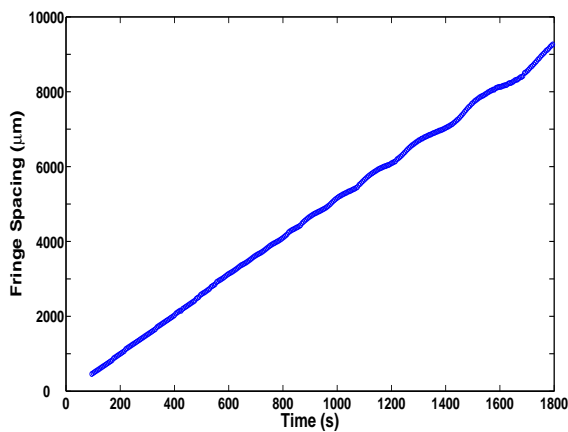
Figure 15: Oil film slope history for Re_\theta = 50,000 in large boundary layer tunnel facility
