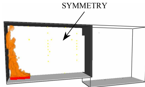
Figure 3. Computational domain of an ISO room fire.
