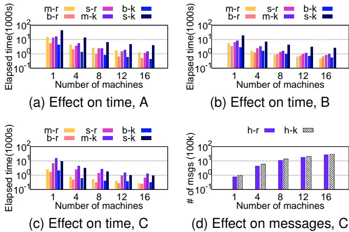
Fig. 7. Scaling out HEADS-JOIN
