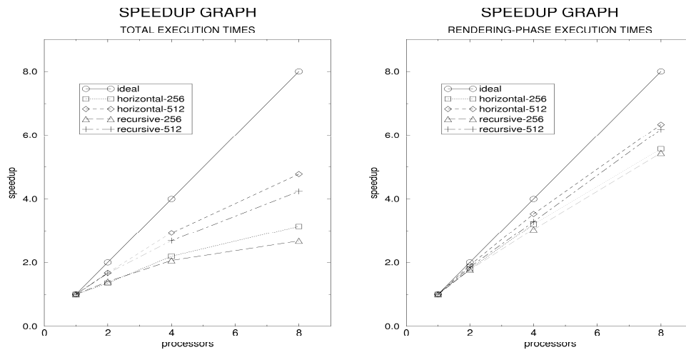
Fig. 3. Speedup graphs of the horizontal and recursive division schemes for total and rendering-phase execution times.
