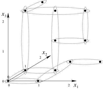
Fig. 1. The one-inclusion hypergraph of Example 9. Vertices are depicted as points, hyperedges as bounding ellipses.
