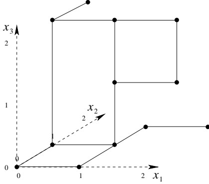
Fig. 7. The graph induced by the one-inclusion hypergraph of Figure 1, for the shifting process in Theorem 52. The graph’s density increases to \frac{14}{12} and pseudo-dimension remains fixed.
