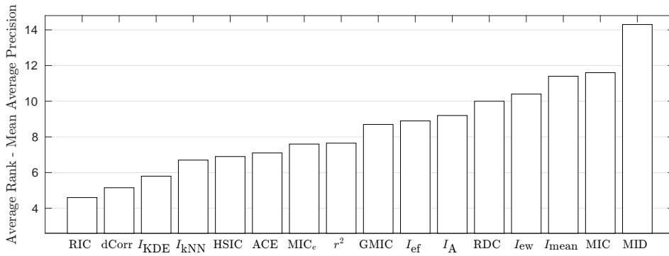
Fig. 12 Average rank across networks on the task of biological network with time inference. RIC outperforms on average all other measures.
