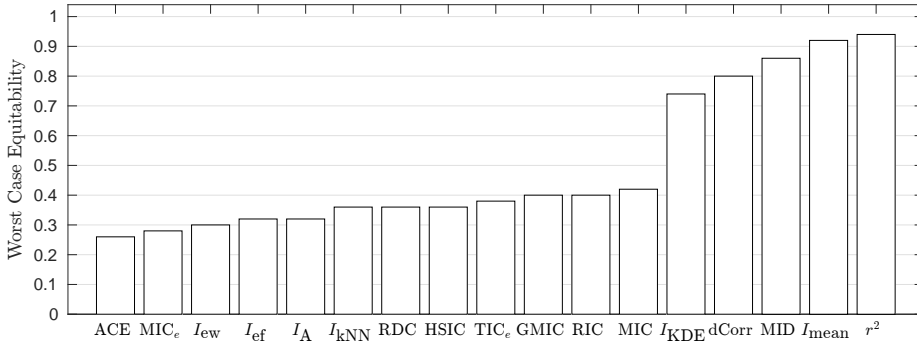
Fig. 10 Worst case equitability for relationships in (Simon & Tibshirani, 2011): i.e. the maximum range of values for R^2 associated to a single value for a measure. That single value corresponds to two completely different levels of noise.
