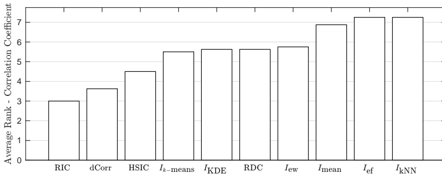
Fig. 17 Average rank when the target is maximization of the correlation coefficient between the predicted and the target value for a k NN regressor. The k NN regression is built on top of m^* features chosen by forward selection. Results are averaged across m^* \leq 10 and all datasets.
