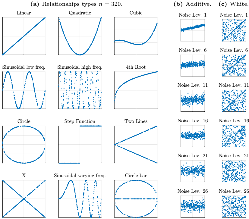
Fig. 5 Relationships between two variables and example of additive and white noise.
