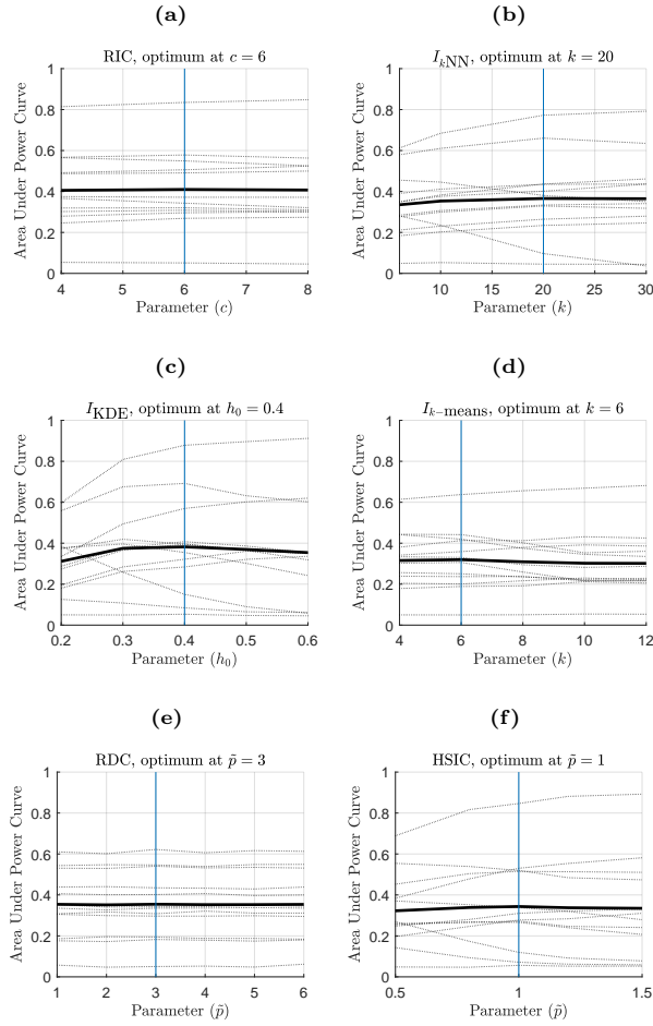
Fig. 22 Parameter tuning to maximize the power of each measure on average for the additive noise model when comparing sets of variables . These plots show the average area under power curve and their average across relationship types.
