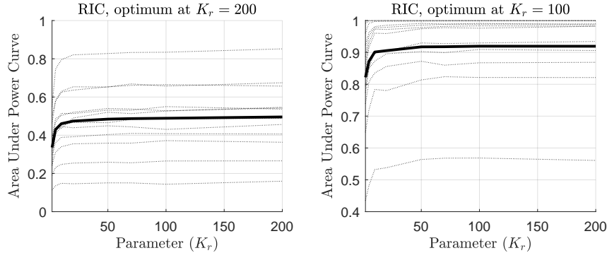
Fig. 6 Each line is the area under the power curve for each relationship tested in this paper. The solid black line shows their average. All results are shown at the variation of the parameter K_r for RIC which determines the number of random discretization grids. The power against independence of RIC always increases at the increase of K_r because its variance decreases. This is particularly important when the number of data points is small: e.g., n = 100 .
