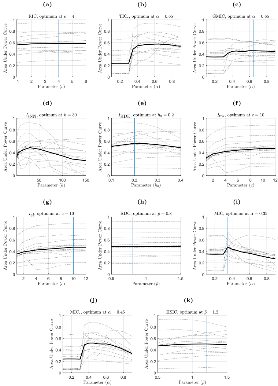
Fig. 18 Parameter tuning to maximize the power of each measure on average for the additive noise model when comparing variables . These plots show the average area under power curve and their average across relationship types.
