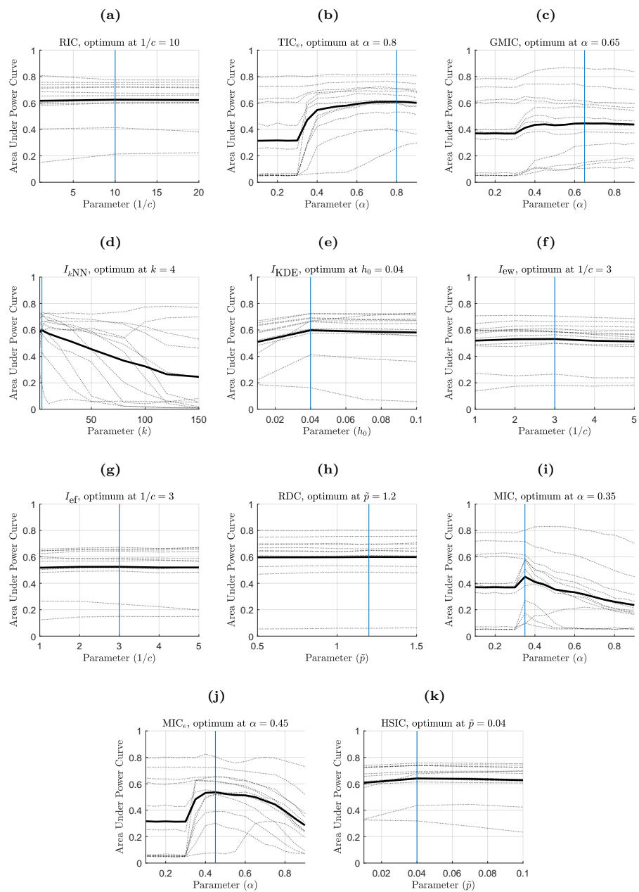
Fig. 19 Parameter tuning to maximize the power of each measure on average for the white noise model when comparing variables . These plots show the average area under power curve and their average across relationship types.
