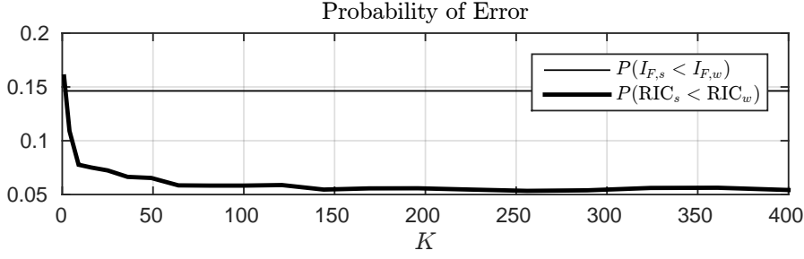
Fig. 3 Probability of error in identifying the strong relationship. RIC's probability is smaller due to its small variance.
