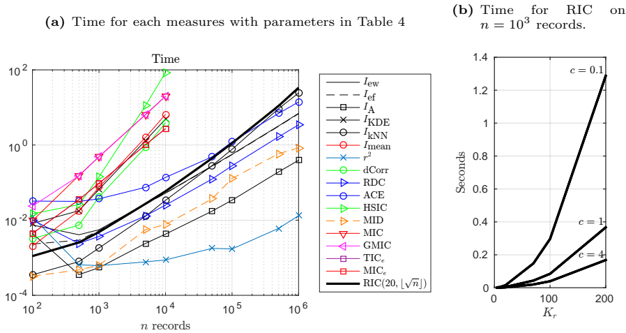
Fig. 14 Running time in seconds (best viewed in color).
