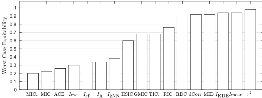
Fig. 11 Worst case equitability for relationships in (Reshef et al., 2011): i.e. the maximum range of values for R^2 associated to a single value for a measure. That single value corresponds to two completely different levels of noise..
