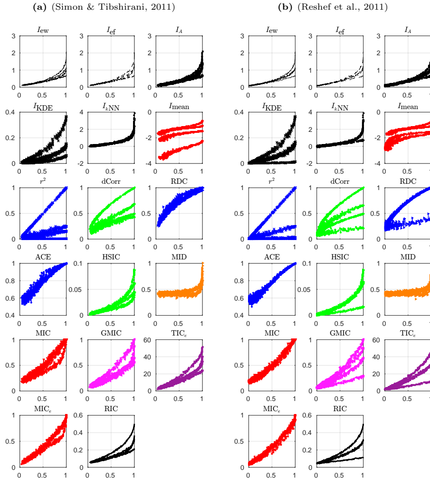
Fig. 9 Equitability of each measure on the two different sets of functional relationships from Table 5. Different values for the R^2 between the noiseless functional relationship and its noisy version are plotted against the value the dependency measure would obtain for that particular amount of noise. The narrower the scatter-plot is, the better the equitability.
