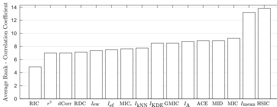
Fig. 13 Average rank of measures when the task is maximizing the correlation coefficient between the predicted and the target value of a k NN regressor. The k NN regression is built on top of m^* features. Results were averaged across m^* \leq 10 and all datasets.
