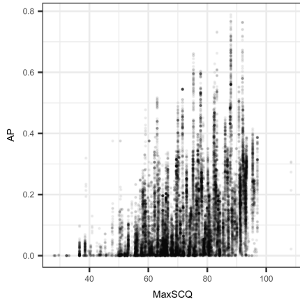
Figure 1: Relationship between MaxSCQ and AP scores, for the 28,869 query:task:ranker triples in UQV100 ( r = 0.42 ).
