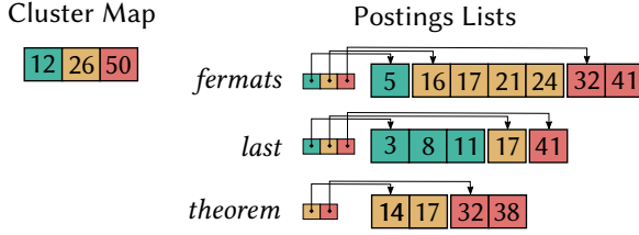
Fig. 3. Postings list arrangement for three possible query terms, “ fermats ”, “ last ”, and “ theorem ”. In addition to the postings lists, a global cluster map stores the last document identifier in each range. Note that the postings list range “pointers” are not required in practice (figure adapted from Hafizoglu et al. [24]).
