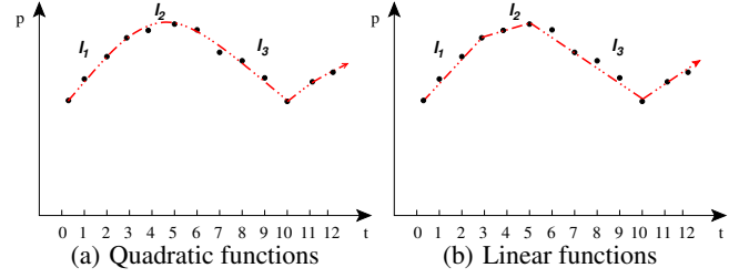
Figure 8: Running example of the AA algorithm
