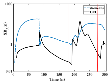
(b) GSA: Gas Sensor Array. Vertical lines indicate the times where concentration of gases change
