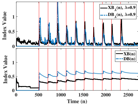
Fig. 4. Values of XB(n) , DB(n) , XB_\lambda(n) and DB_\lambda(n) with \lambda = 0.9 in OEC clusters of the S2 dataset.
