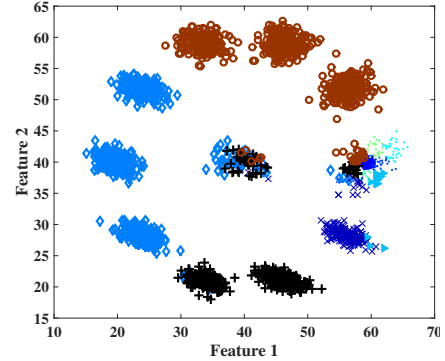
(b) S3: Circular Shifting Gaussian Distribution with Systematic Noise
