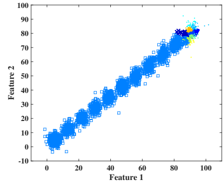
(a) S2: Shifting Gaussian Distribution
