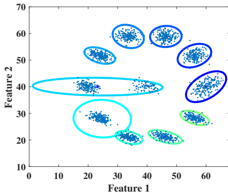
Fig. 7. Terminal OEC clusters on S3 dataset.
