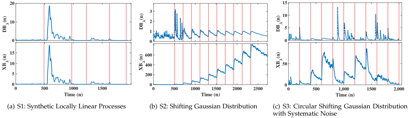
Fig. 5. Values of XB_\lambda(n) and DB_\lambda(n) , \lambda = 0.9 , for sk-means. The vertical lines (red) are times when a change occurs in the dataset.
