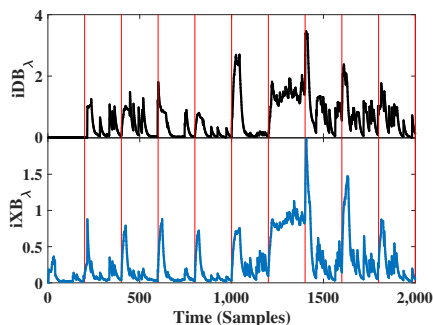
Fig. 8. XB_\lambda(n) and DB_\lambda(n) values for OEC clusters in S3
