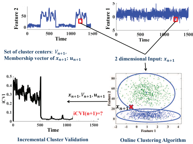
Fig. 1. One-step update of incremental CVI in an online setting.
