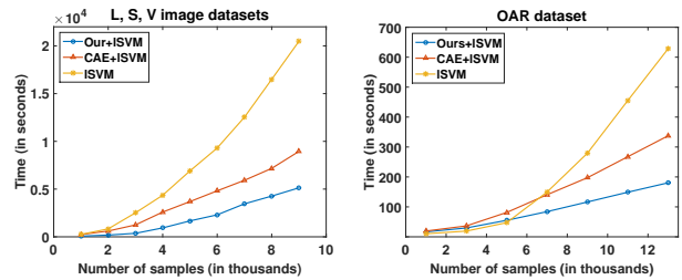
Figure 3: Comparison of the training time of our algorithm with CAE and l -SVM.
