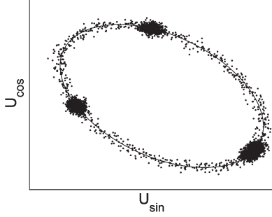
Fig. 4. Example of the distribution of resolver outputs around its characteristic curve. The lumped data points correspond with the resting periods during which the actuator stops or moves slowly.
