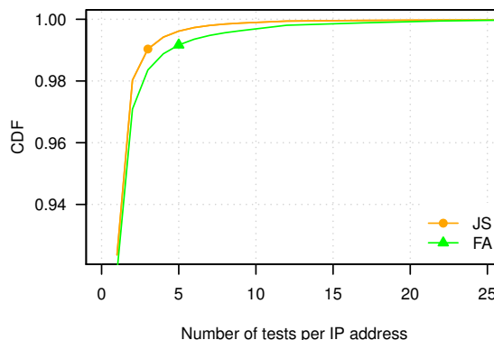
Figure 3: Number of tests per day per IP address for JS-test and FA-test
