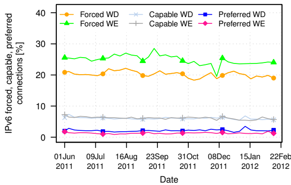
Figure 15: Percentage of IPv6-forced, IPv6-capable and IPv6-preferred for JS test (left) and FA test (right)
