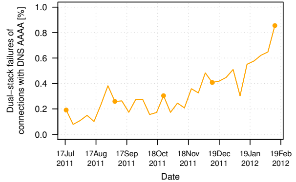
Figure 19: Percentage of connections with DNS AAAA requests with dual-stack failure due to IPv6 problems (upper bound)
