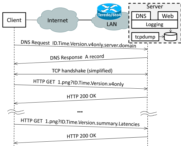
Figure 1: Experimental setup
