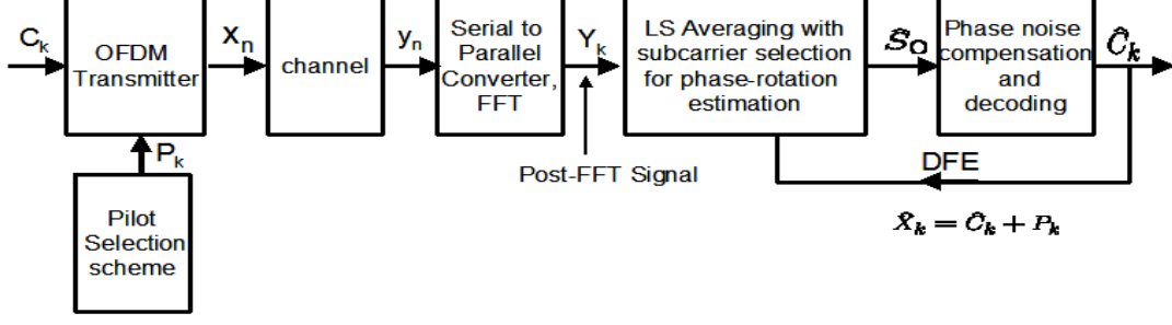
Fig. 3. The OFDM transmission system incorporating the proposed phase-error estimation technique.
