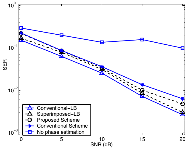
Fig. 5. SER performance of the superimposed scheme with the conventional scheme for BPSK modulation.
