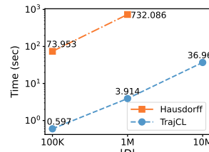
Fig. 6: k NN query costs
