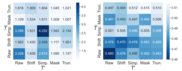
(a) Mean rank ( \blacktriangledown , |D|=100K ) (b) HR@5 ( \blacktriangle , with fine-tuning)
