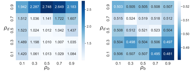
(a) Mean rank ( \blacktriangledown , |D|=100K ) (b) HR@5 ( \blacktriangle , with fine-tuning)
