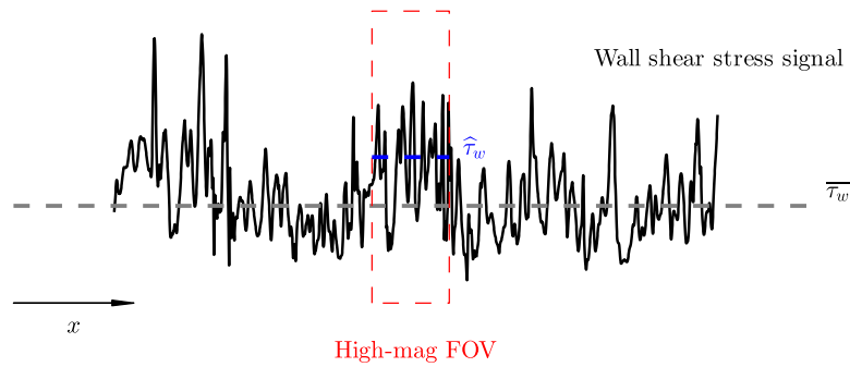
FIG. 10. Schematic showing a sample wall shear stress signal evolving with x . The dashed red box corresponds to the streamwise length of the high-mag FOV. The corresponding local mean \hat{\tau}_w is shown by a blue dashed line and the global mean ( \bar{\tau}_w ) is represented by the grey dashed line.
