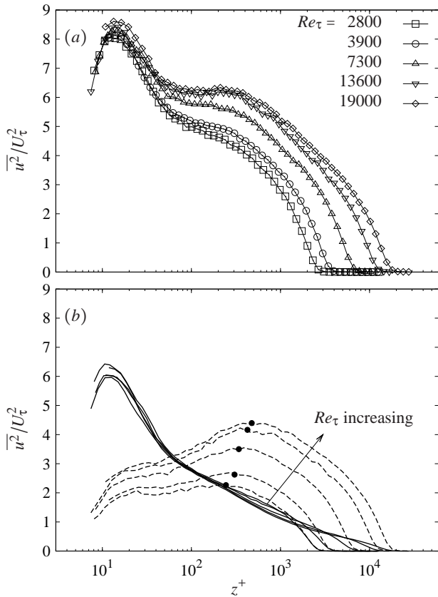
Figure 1: (a) Reynolds number dependency of the streamwise turbulence intensity profiles \overline{u^2}/U_\tau^2 ; (b) Decomposition of the streamwise turbulence intensity profile into small-scale ( \lambda_x^+ < 7000 , solid lines) and large-scale components ( \lambda_x^+ > 7000 , dashed lines), the sum of both components is equal to profiles in figure (a).
