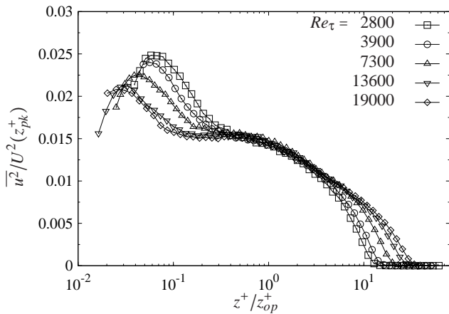
Figure 4: Scaling of the total streamwise turbulence intensity by the local mean velocity at the outer-peak U^2(z_{pk}^+) versus z^+/z_{op}^+ .
