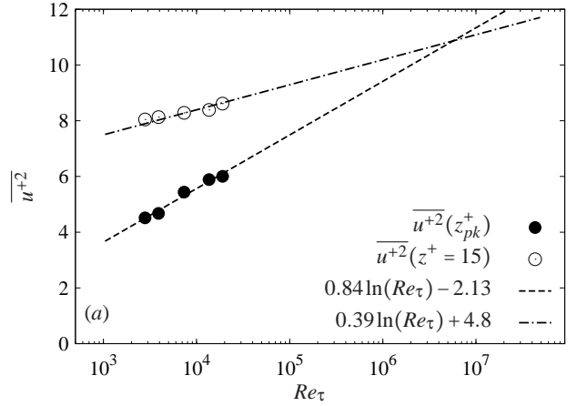
Figure 3: Reynolds number dependency of the total streamwise turbulence intensity at the inner- ( \circ ) and outer-peak ( \bullet ) locations; The dotted-dashed line and the dashed line are the respective log-law curve fits.
