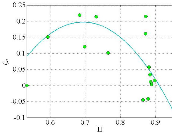
Figure 6: Experimental data of this study. The solid line corresponds to equation (17).
