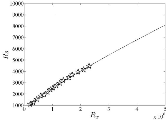
Figure 5: Evolution of momentum thickness Reynolds number ( R_\theta ) for different streamwise Reynolds number ( R_x ). Star ( \star ) symbols represent the experimental data points, the solid line corresponds to evolution calculations with same initial conditions as the experimental data.
