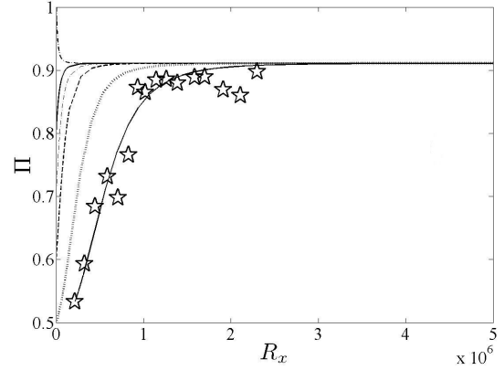
Figure 3: Evolution of wake parameter ( \Pi ) for different streamwise Reynolds number ( R_x ). Star ( \star ) symbols represent the experimental data points, the solid line corresponds to evolution calculations with same initial conditions as the experimental data and dotted lines correspond to evolution calculations with different initial conditions
