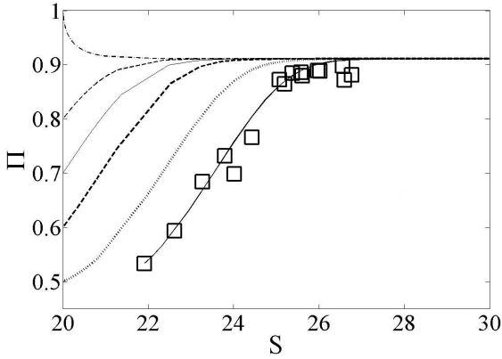
Figure 2: Evolution of wake parameter ( \Pi ) for different Non dimensionalised free stream velocity ( S ). Box ( \square ) symbols represent the experimental data points, the solid line corresponds to evolution calculations with same initial conditions as the experimental data and dotted lines correspond to evolution calculations with different initial conditions.
