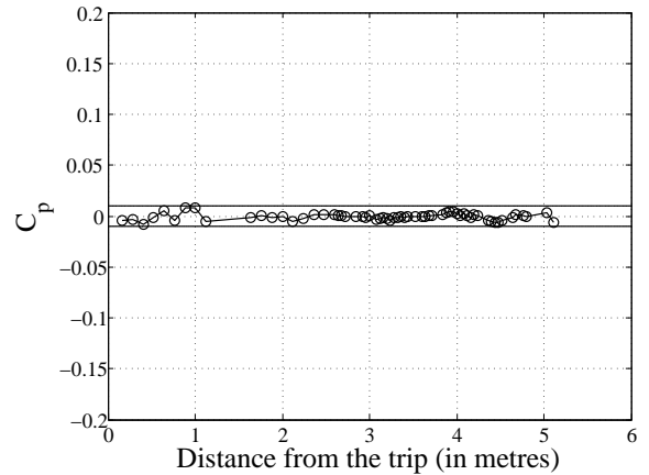
Figure 1: Co-efficient of pressure ( C_p ) along the wind tunnel .
