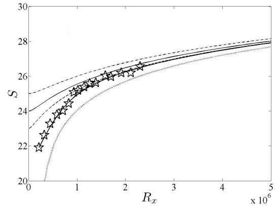
Figure 4: Evolution of skin friction factor ( S ) for different streamwise Reynolds number ( R_x ). Star ( \star ) symbols represent the experimental data points, the solid line corresponds to evolution calculations with same initial conditions as the experimental data and dotted lines correspond to evolution calculations with different initial conditions
