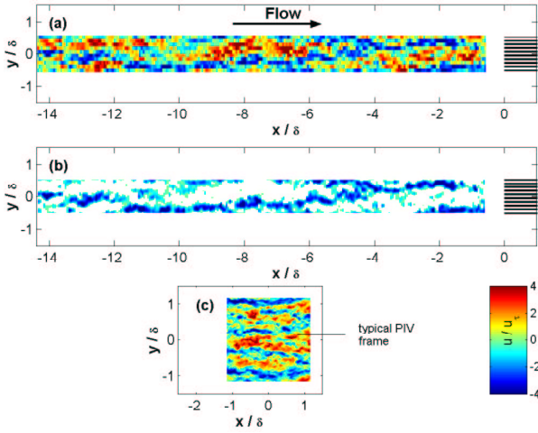
Figure 6: (a) Example signal section from ten sensor hot-wire rake at z/\delta = 0.14 . Spatial view is reconstructed using local mean velocity ( x = -U_{ct} ); (b) the negative momentum fluctuations only; (c) comparison with typical PIV frame.
