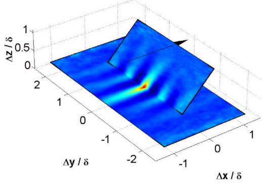
Figure 5: R_{III} calculated from datasets (i) & (ii) at z_{ref} = 0.14\delta for the mode 0.5 < \lambda_y/\delta < 0.75
