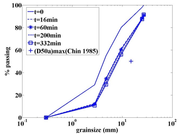
Figure 2. Change in grading curve over duration of experiment.
