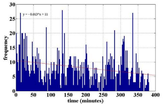
Figure 3. Frequency of particle movements (greater than the maximum particle diameter) over the duration of the experiment.
