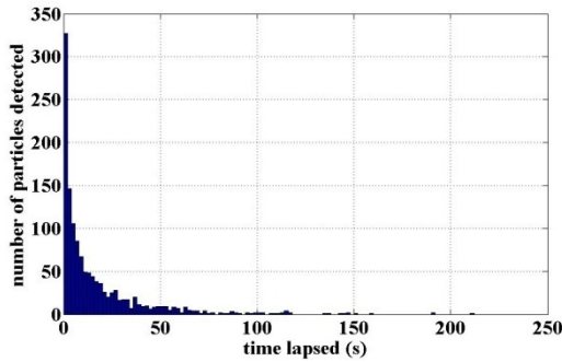
Figure 4. Histogram of the time elapsed between individual particle movements.
