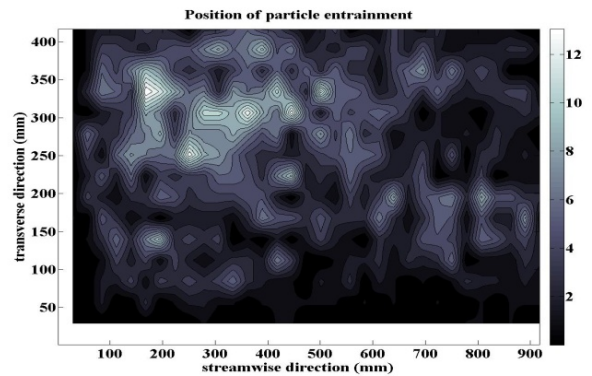
Figure 5. Frequency of position of particle entrainment (number of particles entrained from the bed for the duration of the test. Talled by dividing the bed into a grid)
