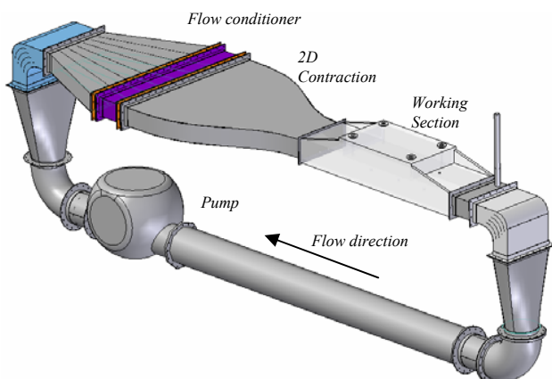
Figure 3. UTAS Water Tunnel Schematic
