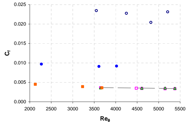
Figure 5. Comparison of local skin friction coefficient data for smooth and fouled test plates. \square Smooth plate (Preston), \triangle Smooth plate (log-law slope), \bullet Barton [3] smooth plate (Preston), \circ Fouled plate (200mm streamers), \diamond Barton [3] fouled plate (30mm streamers), --- Smooth plate equilibrium.
