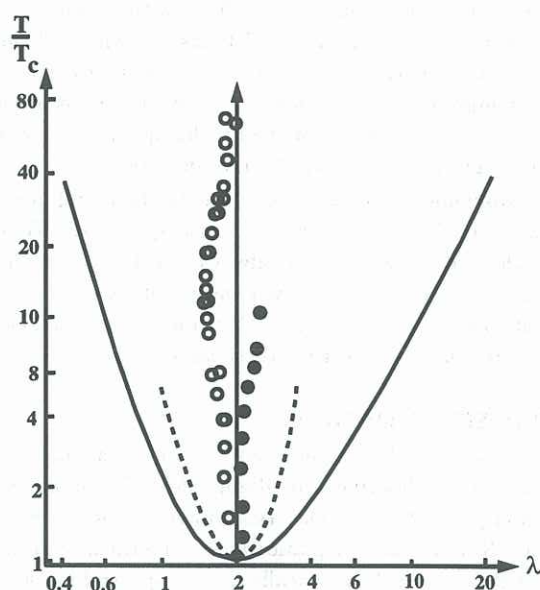
Figure 1: Stability diagram for Taylor vortex flow for \eta = 0.727 , \mu = 0 . Taylor number versus axial wavelength. The solid line is the neutral curve from the linear stability of steady circular Couette flow. The dashed line shows the stability boundary from a weakly nonlinear analysis by Kogelman & DiPrima (1970). The open circles represent Taylor vortex flow states observed for sudden start experiments by Burkhalter & Koschmieder (1974). The solid circles represent Taylor vortex flow states observed for an experiment where the annulus was filled with fluid after inner cylinder was rotating at fixed speed. From Burkhalter & Koschmieder (1974).
