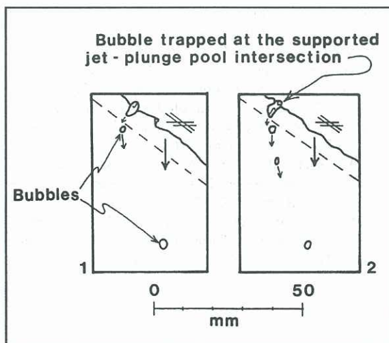
Fig. 4: Air bubble entrainment caused a trapped surface bubble. Flow direction from top to bottom : V = 1.20 m/s, Tu = 1.08\% , d = 8.0 mm, L_j = 34 mm. Video shutter speed : 1.0 ms, frame interval : 20 ms.
