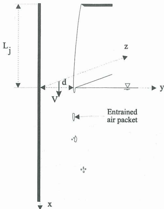
Fig. 1: Sketch of the experiment
