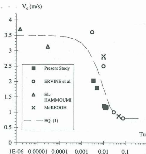
Fig. 2: Inception velocity of air entrainment
