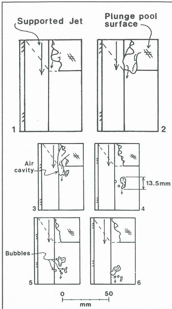
Fig. 3: Elongated air cavity formation and entrainment of bubbles. Flow direction from top to bottom : V = 1.20 m/s, Tu = 1.08\% , d = 8.0 mm, L_j = 34 mm. Video shutter speed : 1.0 ms, frame interval : 20 ms
