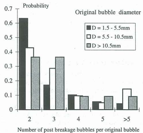
Fig. 5: Single bubble breakage : number of breakage products per original bubble
