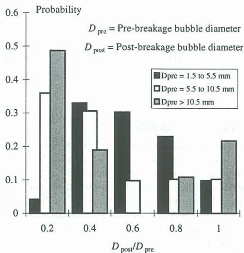
Fig. 6: Single bubble breakage : dimensionless post-breakage bubble size
