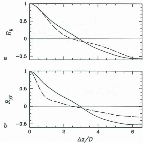
Figure 4: Comparison of spanwise autocorrelations for the fixed (---) and oscillating (—) cylinders. Autocorrelations of (a), lift force; (b), out-of-plane velocity ( v ) on the centre plane, 20D downstream.
