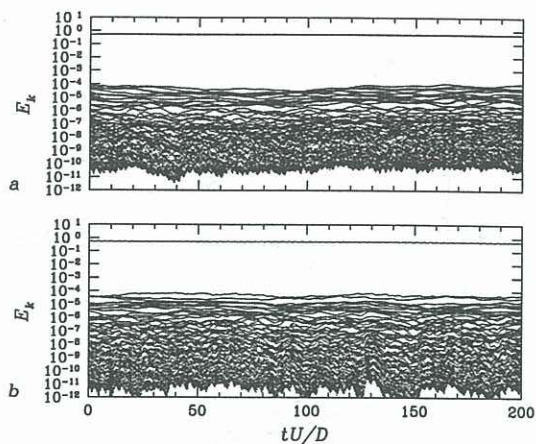
Figure 5: Time series of modal energies E_k for (a) fixed and (b) oscillating cylinder. The dominant value is for the mean flow, E_0 \approx 0.5 , while the lower values E_k < 1 \times 10^4 are for the remaining modes 1 \leq k < 72 .
