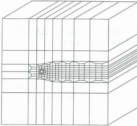
Figure 1: Computational mesh with 218 spectral/Fourier elements. The domain is 37.5 D in streamwise extent, 40 D in cross flow extent and 13.12 D in spanwise extent.
