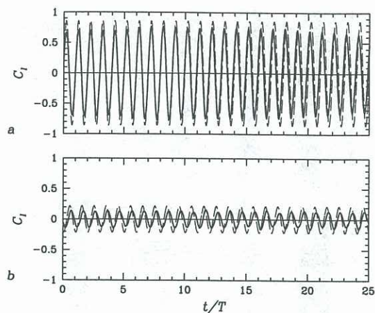
Figure 6: Time series of coefficient of lift. (a): Cylinder fixed, timebase normalised with vortex shedding period (average value in three-dimensional case). (b) Oscillating cylinder, timebase normalised with cylinder oscillation period. —, three-dimensional flow; - -, two-dimensional flow.
