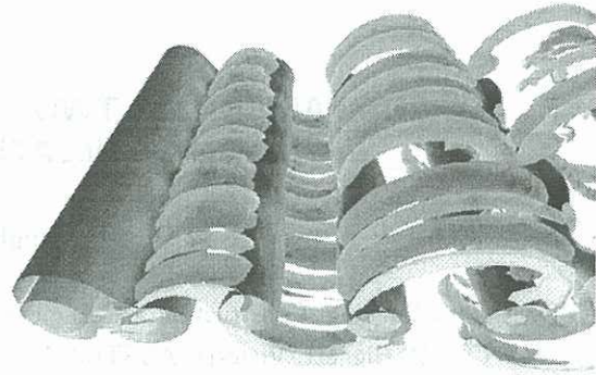
Figure 2: Flow past a fixed circular cylinder (left) at Re = 265 . Isosurfaces of pressure (aligned mainly spanwise) and streamwise vorticity (aligned mainly streamwise).
