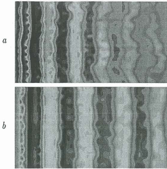
Figure 3: Contours of out-of-plane velocity ( v ) on the wake centre plane for a circular cylinder at Re = 265 . (a): Cylinder fixed. (b): Cylinder forced to oscillate cross-flow at 78% of the Strouhal frequency for the fixed cylinder, y_{max}/D = 0.25 .
