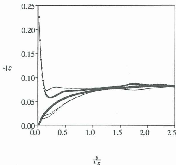
FIGURE 2. The \epsilon_{11} and \epsilon_{22} components of the dissipation tensor as a function of the distance from the wall. \bullet , \epsilon_{11} from DNS; —, \epsilon_{11} from improved model; - - -, \epsilon_{11} from basic model; \blacksquare , \epsilon_{22} from DNS; - - -, \epsilon_{22} from the improved model; \cdots , \epsilon_{22} from the basic model; ( T_E = 3 , Re_\lambda = 65 , L_E = \frac{q^{3/2}}{\epsilon} )
