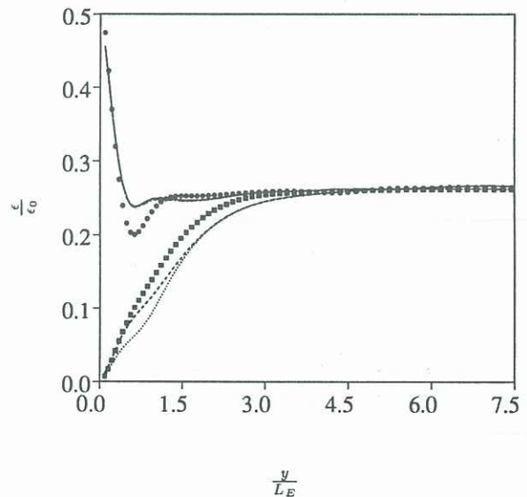
FIGURE 1. The \epsilon_{11} and \epsilon_{22} components of the dissipation tensor as a function of the distance from the wall. \bullet , \epsilon_{11} from DNS; —, \epsilon_{11} from improved model; - - -, \epsilon_{11} from basic model; \blacksquare , \epsilon_{22} from DNS; \cdots , \epsilon_{22} from the improved model; \cdot\cdot\cdot , \epsilon_{22} from the basic model; ( T_E = 1 , Re_\lambda = 15 , L_E = \frac{q^{3/2}}{\epsilon} )
