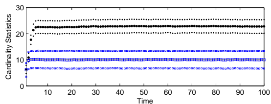
Fig. 10. True cardinality (solid line) shown versus estimated mean cardinality and corresponding standard deviation for the MeMBER filter ( \bullet/\bullet ) and similarly for the PHD filter ( o/o ). The MeMBER filter is biased but the PHD filter is unbiased.
