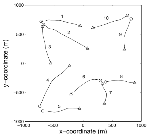
Fig. 4. True tracks in the xy plane. Targets move with non-constant velocity along the paths shown. Start/Stop positions are shown with \circ/\Delta .
